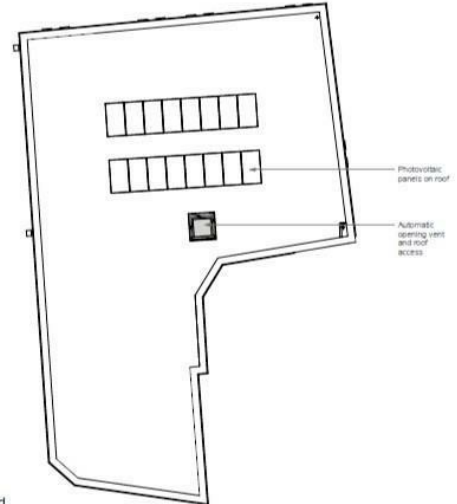
03-Roof Level Proposed 1:100
